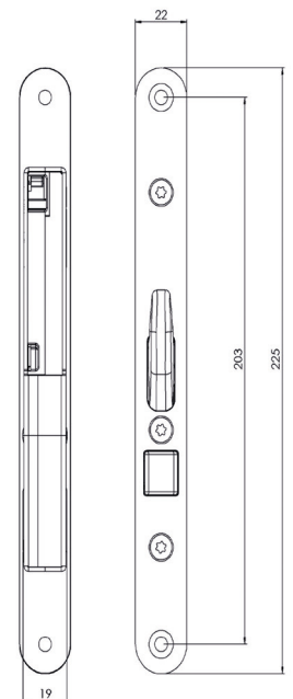
Dimensional drawing for STEP 552.
