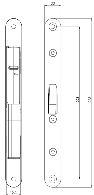
Dimensional drawing for H51.
